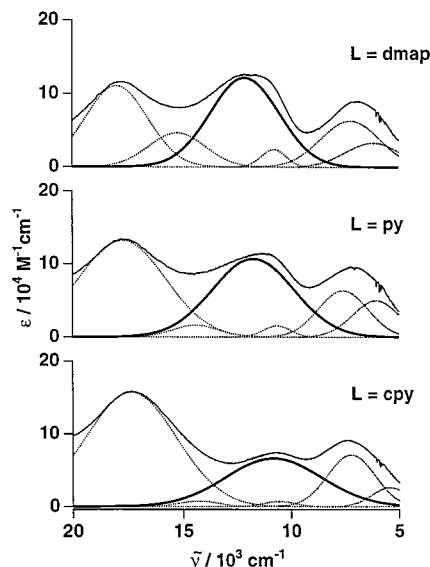
Figure 4. Electronic absorption spectral data for 1 (top), 2 (middle), and 3 (bottom) in the 1-electron reduced ( n = -1 ) states in dichloromethane, -10 °C (solid line), and the deconvoluted ICT band (dotted line). The solid bold line corresponds to the single Gaussian fit of the ICT band.
